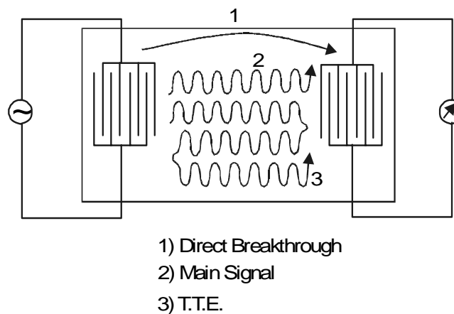
Figure 90: SAW Filter Signal Paths
