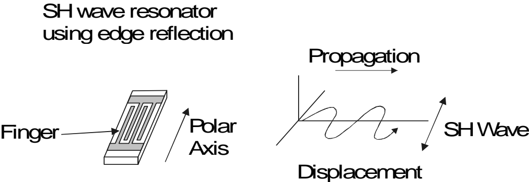
Figure 107: BGS and SH Wave Resonators
