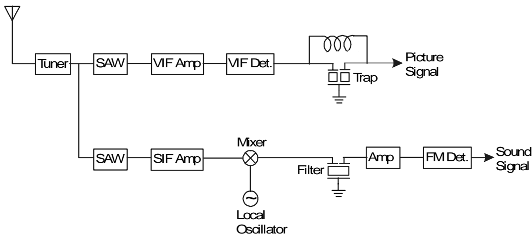
Figure 97: Split-Carrier System
