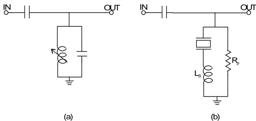
Figure 69: Discriminator Circuit
