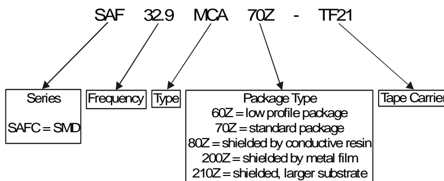
Figure 103: SAW Filter Part Numbering System
