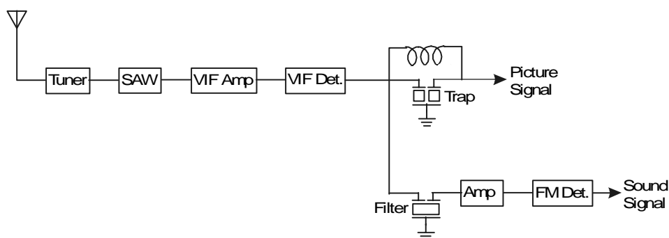
Figure 49: Inter-Carrier System
