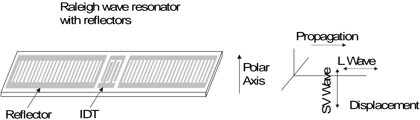
Figure 105: Rayleigh Wave Resonator
