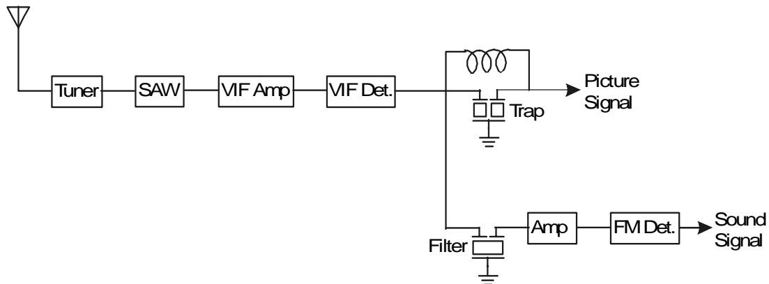
Figure 95: Inter-Carrier System
