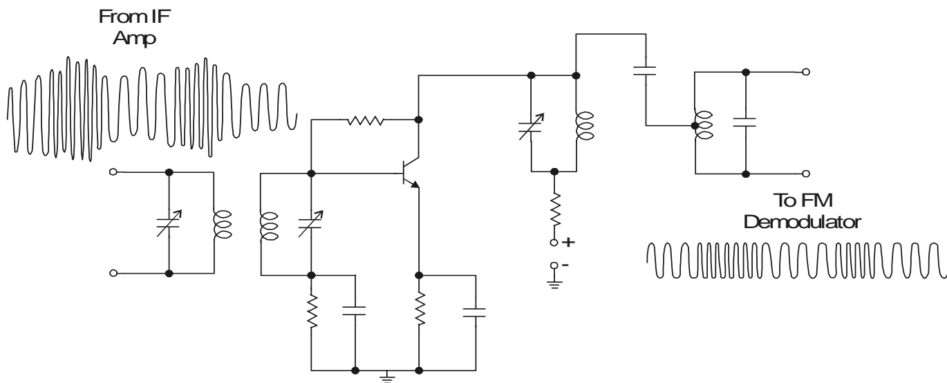
Figure 65: Limiter Circuit
