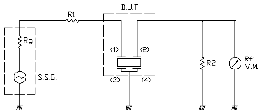
FIGURE 2 TEST CIRCUIT
