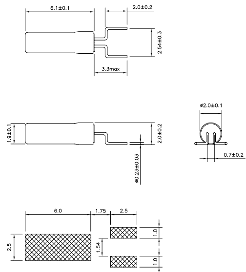
PCB PAD LAYOUT RECOMENDATION
