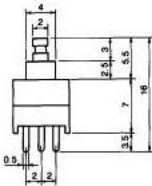
Mounting
