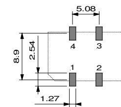
PC board footprint
