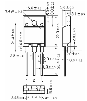
TO-3PML
