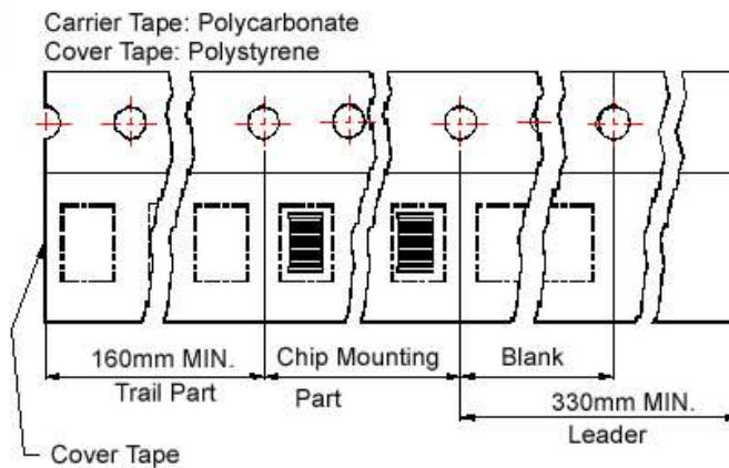
Tape Material
