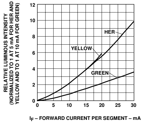
Figure 9. Relative Luminous Intensity vs. DC Forward Current.
