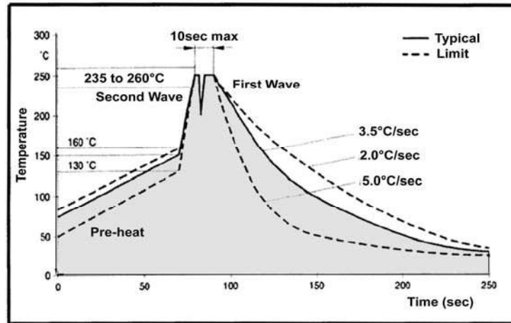
Fig. 3 Recommended Wave Soldering Profile
