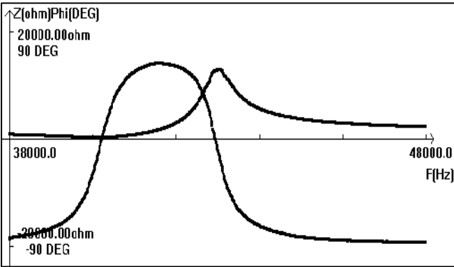
Transmitter impedance
