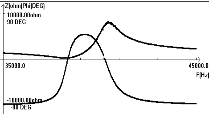
Receiver impedance
