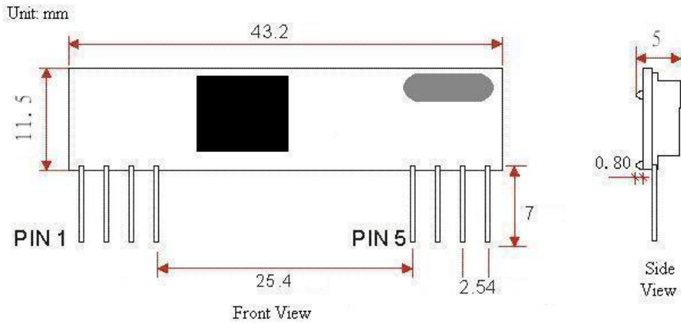
Figure2 CY07-V1.1 Dimension
