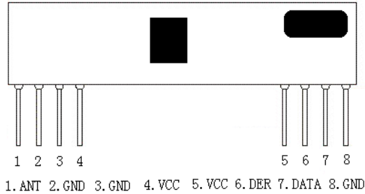
Figure1 CY07-V1.1Shape & Pins
