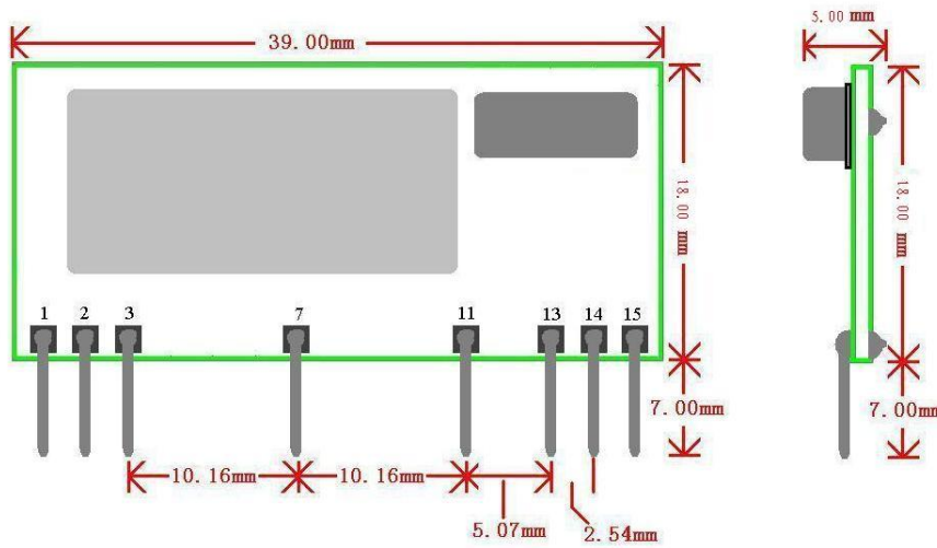
Figure2 CY58 Dimension
