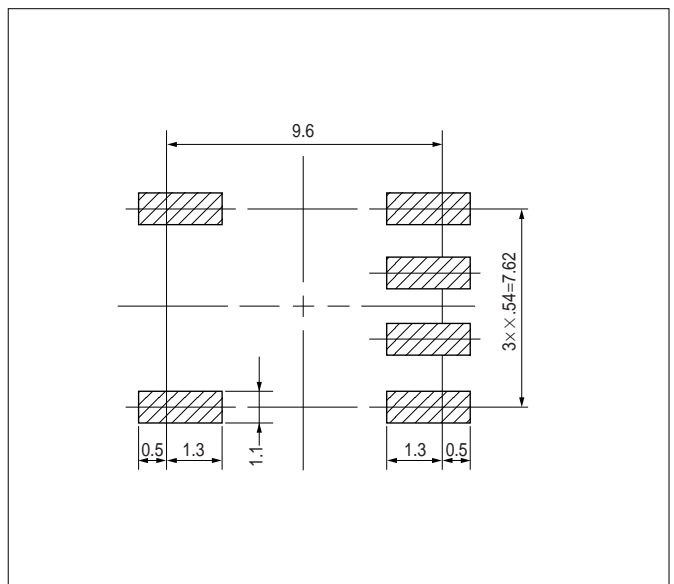
Dimensions(mm)
