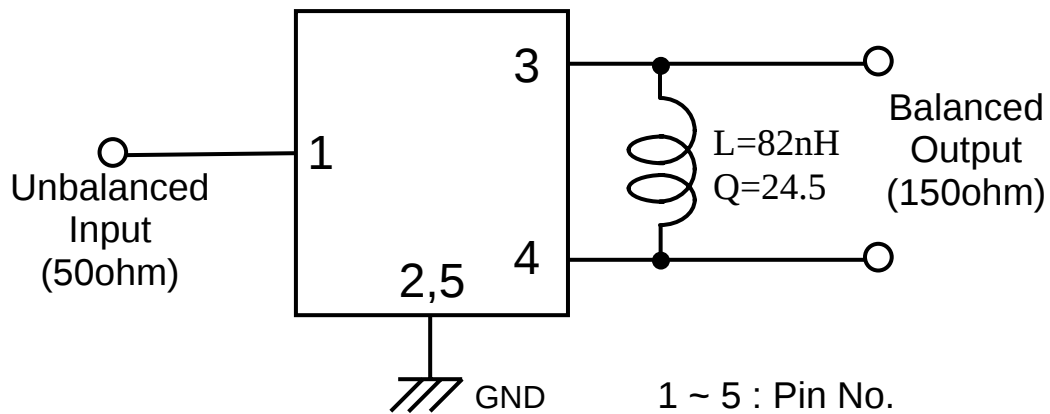
Fig.2 Evaluation circuit
