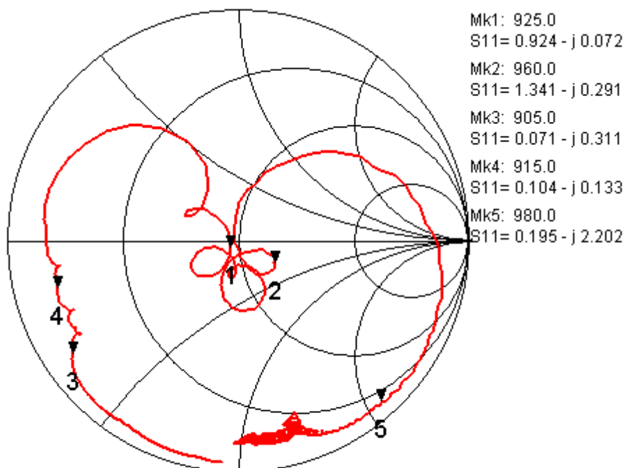
Impedance S11(Unbalanced)
