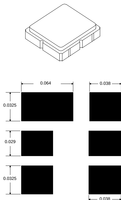
PCB Foot Print Dimensions in Nominal Inches
