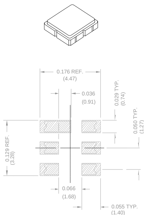
PCB Footprint
