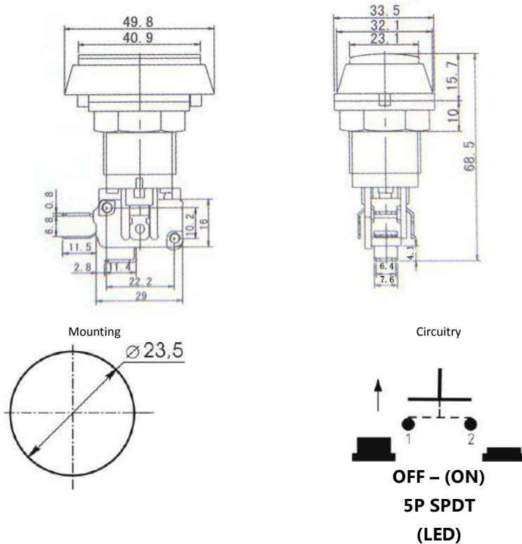
Outline Drawing
