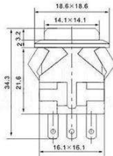
Outline Drawing
