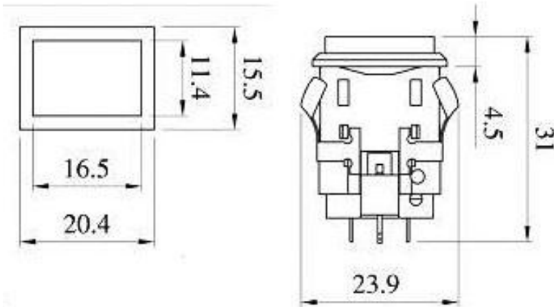
Mounting
