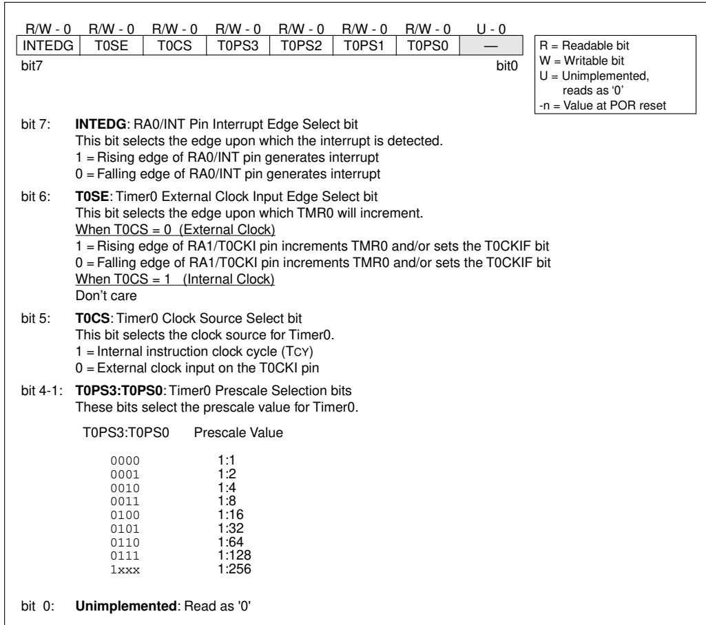
FIGURE F-3: T0STA REGISTER (ADDRESS: 05h, UNBANKED)
