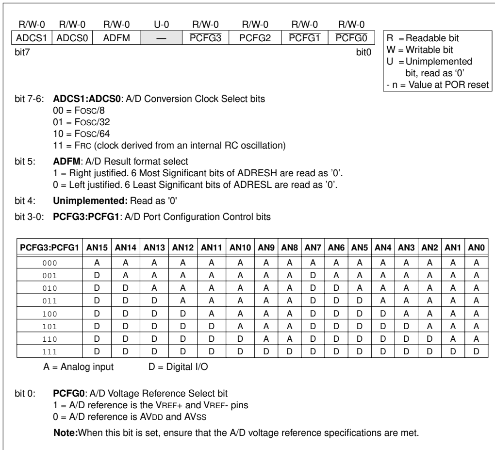
FIGURE F-16: ADCON1 REGISTER (ADDRESS 15h, BANK 5)
