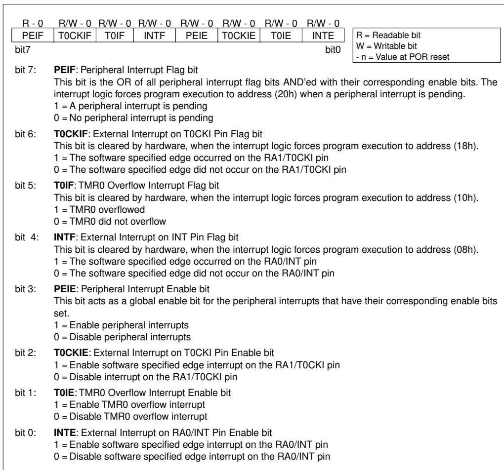
FIGURE 6-2: INTSTA REGISTER (ADDRESS: 07h, UNBANKED)
