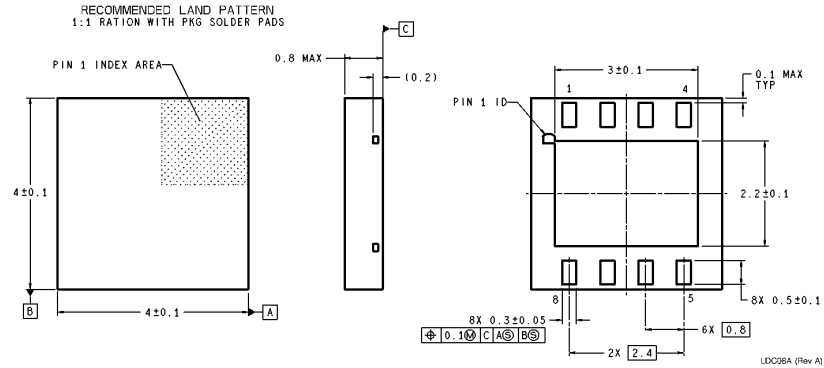
8-Lead LLP Order Number LM2940LD-5.0, LM2940LD-8.0, LM2940LD-9.0, LM2940LD-10, LM2940LD-12 or LM2940LD-15 NS Package Number LDC08A
