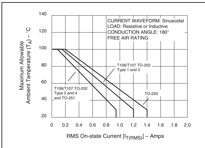
Figure E5.6 Maximum Allowable Ambient Temperature versus RMS On-state Current
