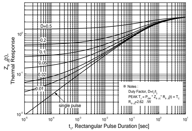
Fig.10 Transient Thermal Response Curve
