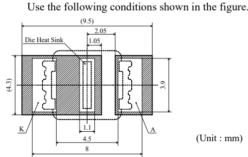
[Recommended soldering pad design]
