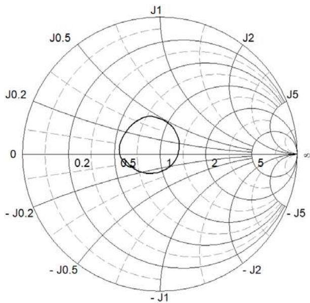
Ant Input Impedance (Tx Band)
