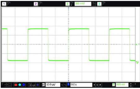
Figure 15. LVC MOS Output Waveform ( V_{swing} = 1.8\text{V} , SiT1534AI-J4-DCC-32.768)
